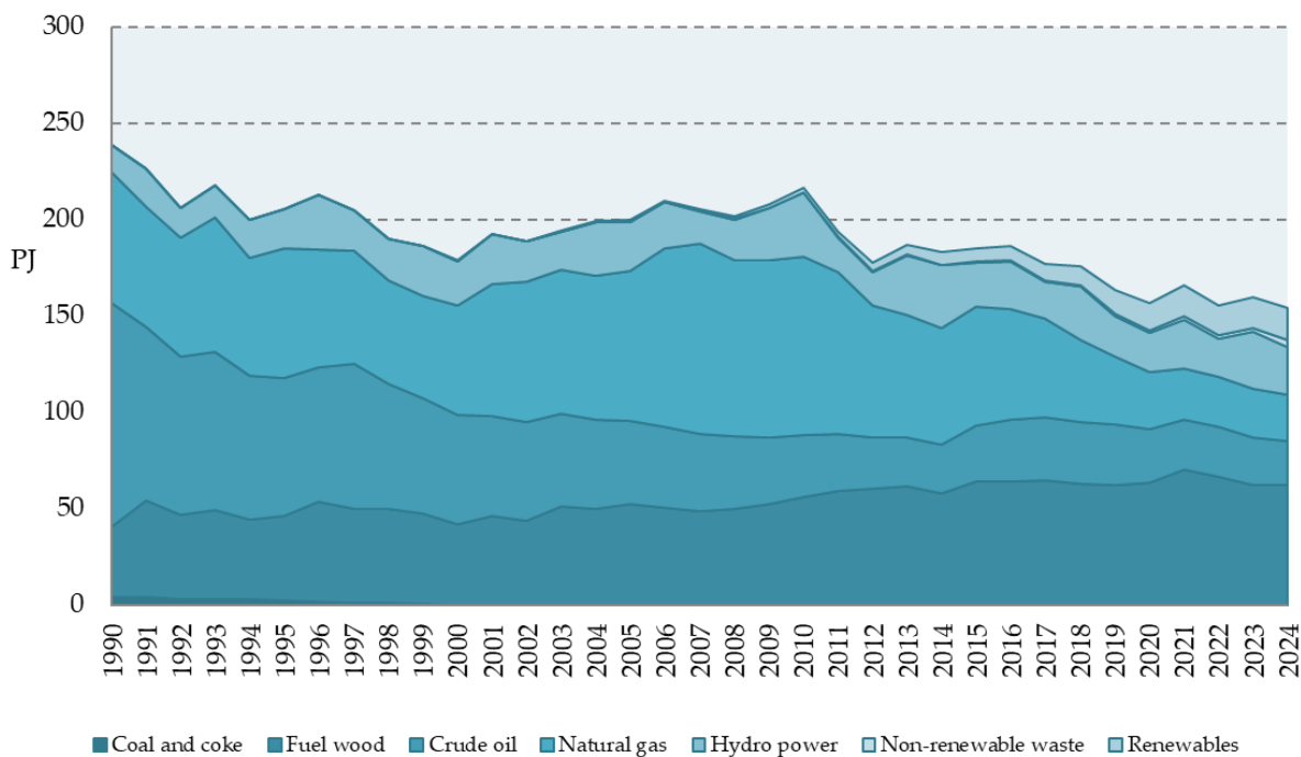
Figure 3.1-1: Trends in primary energy production for the period from 1990 to 2024
