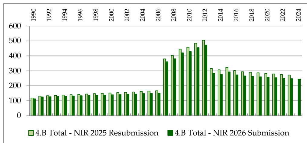
Figure 6.5-1: Current and previously reported emissions for category 4.B (kt CO 2 -eq)
