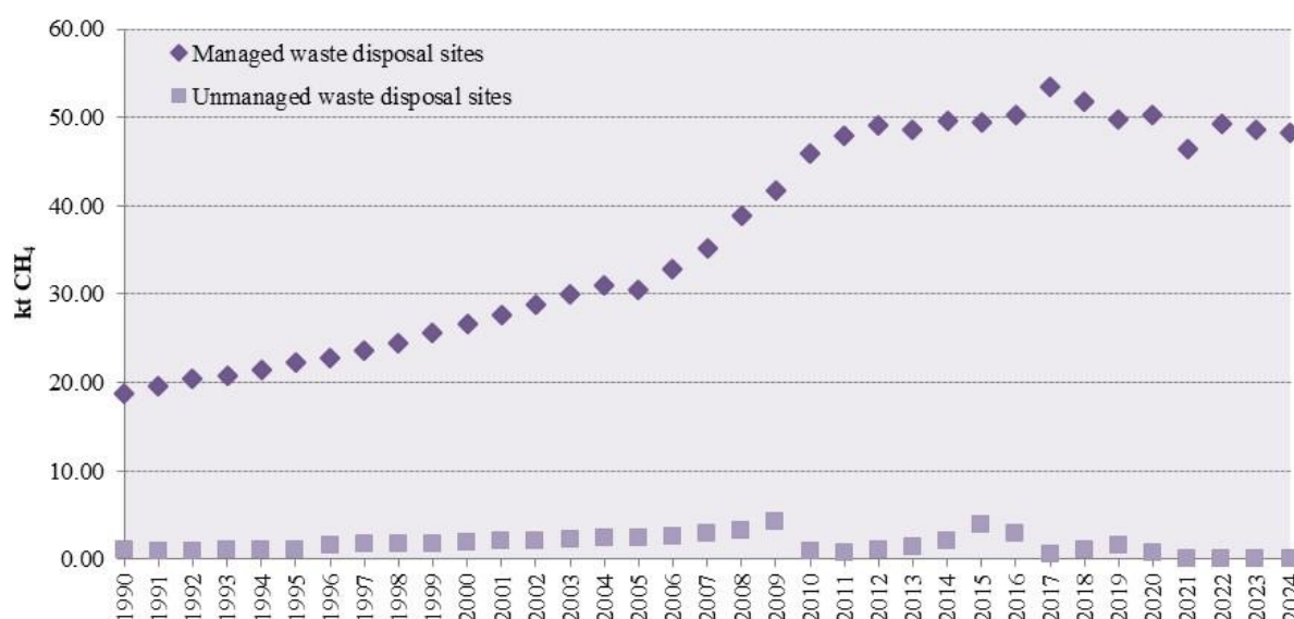
Figure 7.2-2: Trends of CH 4 emissions from managed and unmanaged waste disposal sites (1990 - 2024)
