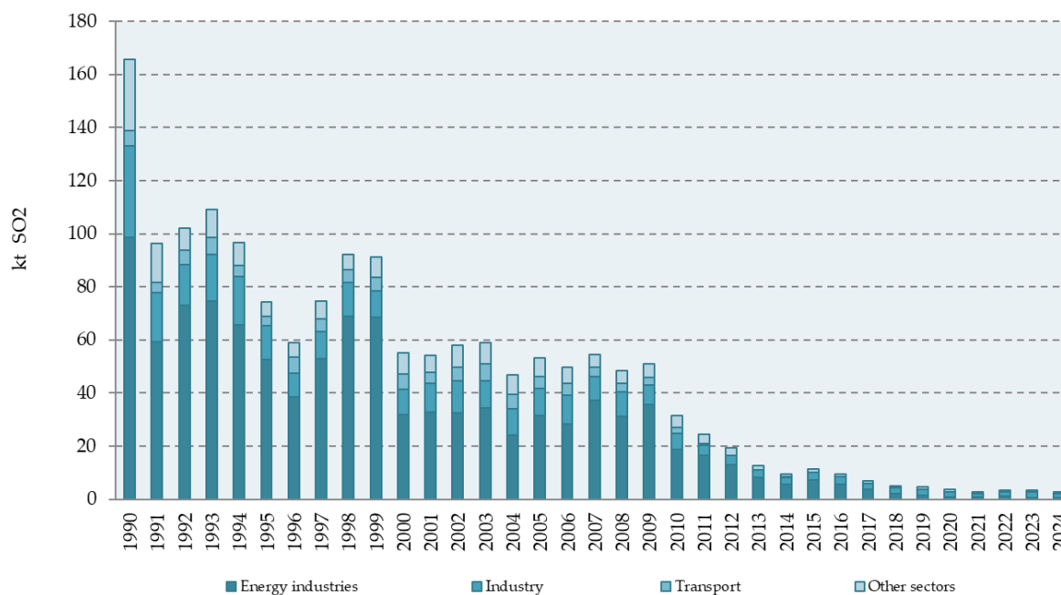
Figure 3.1-10: SO 2 emissions from Energy sector in the period 1990-2024
