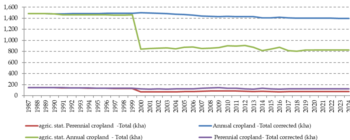
Figure 6.3-13: Area of Annual and Perennial cropland in Croatia after adjustments of CBS data, kha
