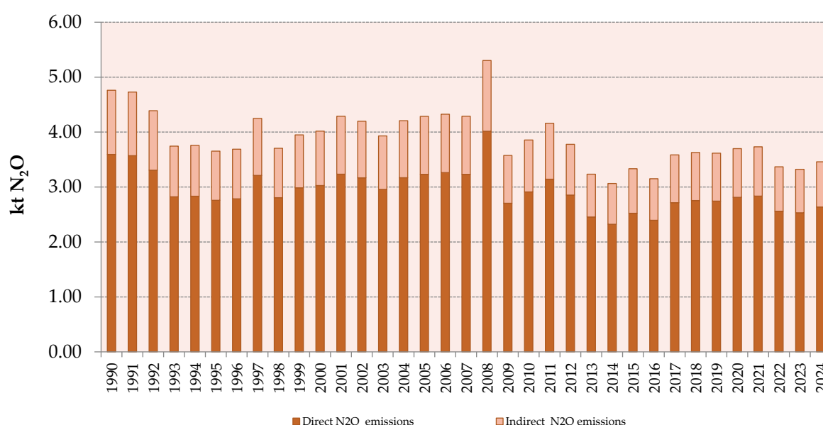
Figure 5.5-1: Total N 2 O emissions from Agricultural soils
