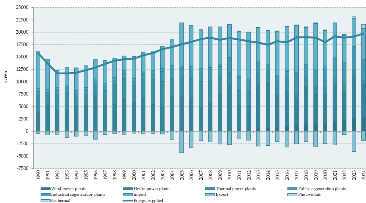
Figure 3.2-2: Electricity supply for the period from 1990 to 2024
