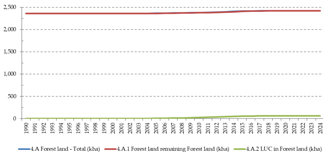
Figure 6.4-1: Trend of Forest land* and LUC to Forest land in period 1990-2024 (kha)
