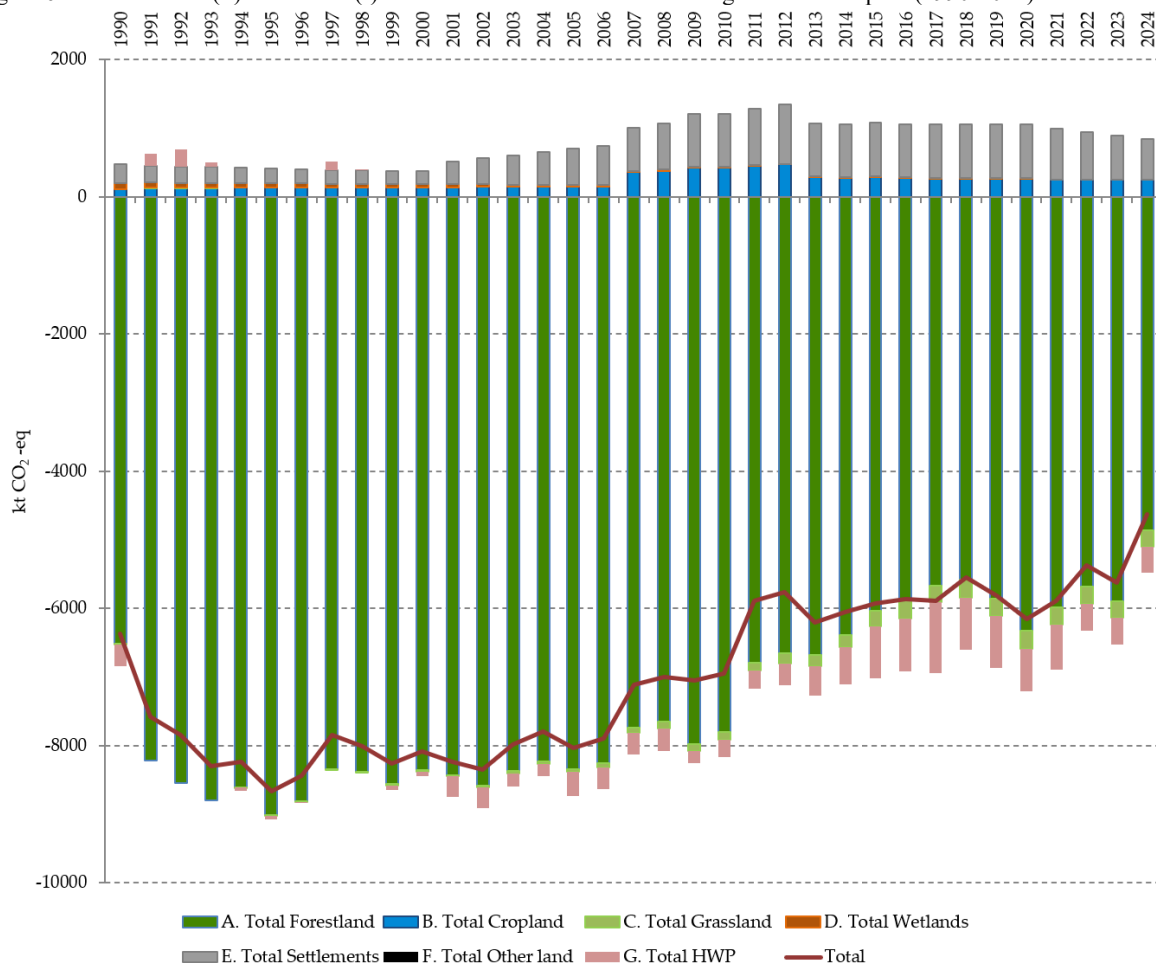
Figure 6.1-1: Emissions (+) / removals (-) trend for LULUCF sector land categories + HWP pool (1990-2024)
