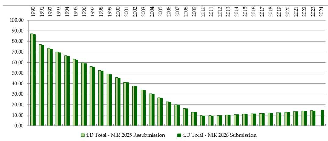
Figure 6.7-1: Current and previously reported emissions for category 4.D (kt CO 2 -eq)
