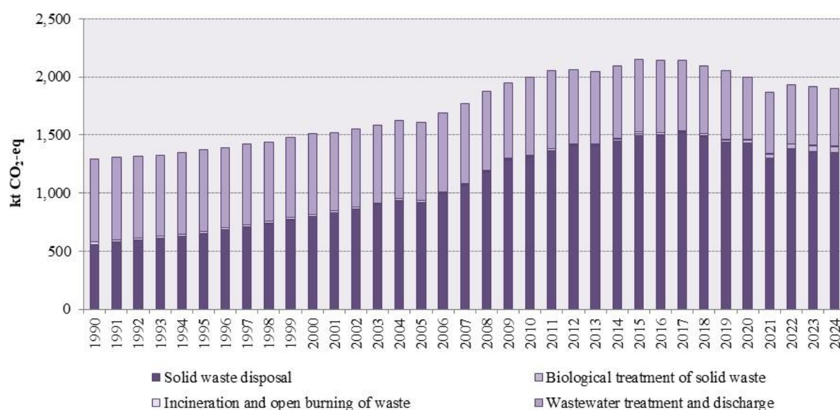
Figure 7.1-1: Emissions of GHGs from Waste sector (1990 - 2024)
