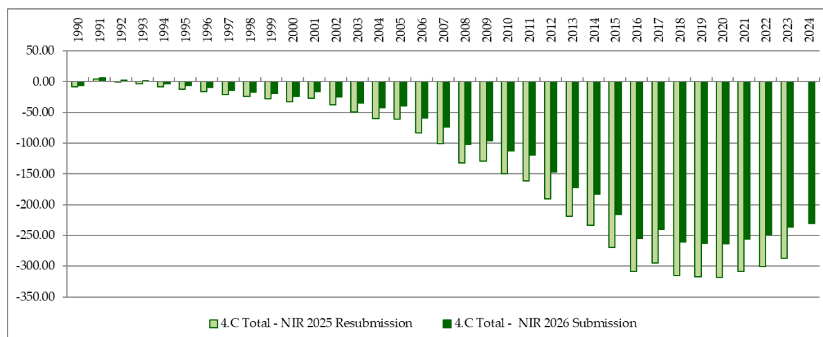
Figure 6.6-1: Current and previously reported emissions for category 4.C (kt CO 2-eq )
