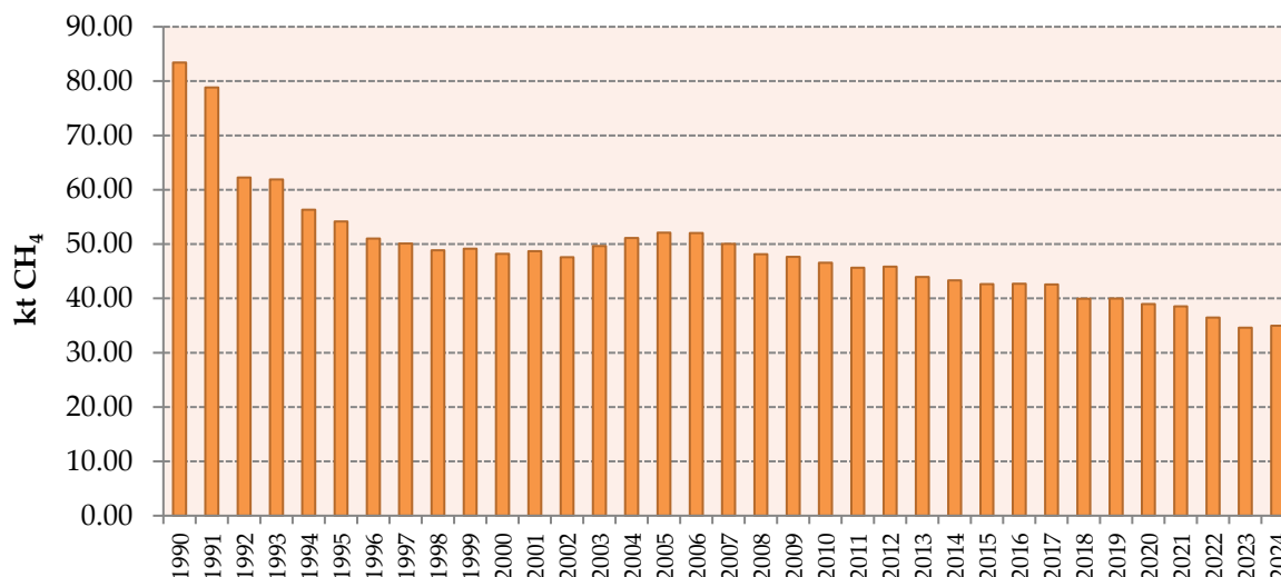
Figure 5.2-1: CH 4 emission from Enteric fermentation
