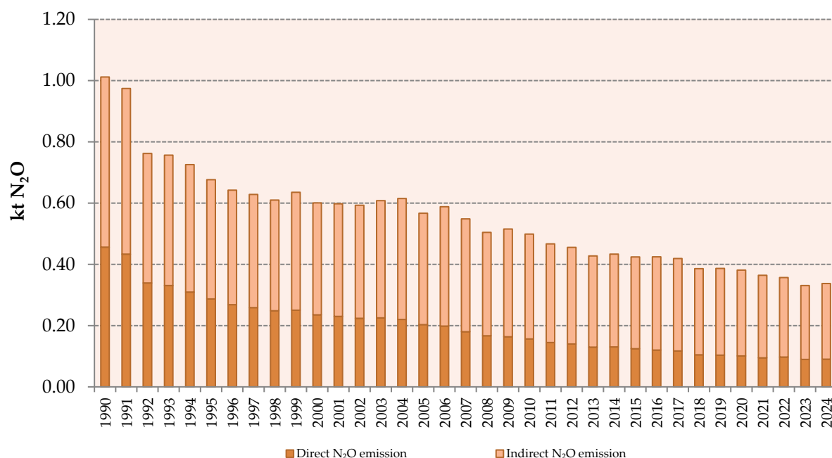
Figure 5.3-2: N 2 O Emissions from Manure management
