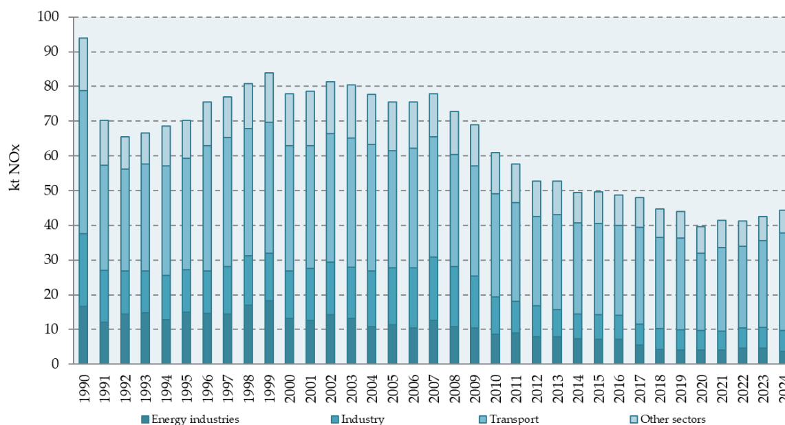
Figure 3.1-7: NO x emissions from Energy sector in the period 1990-2024
