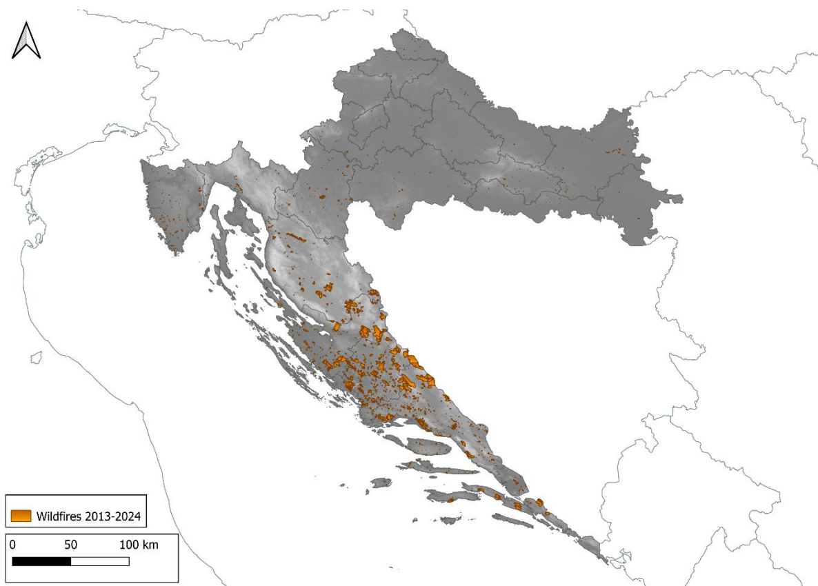
Figure 6.15-4: Spatial distribution of forest fires in Croatia for period 2013-2024
