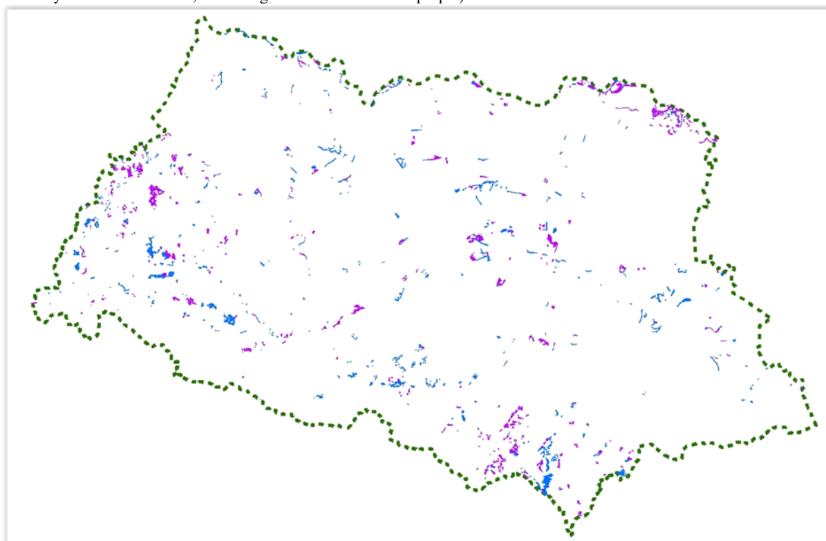
Figure 6.4-12: Forest Administration Našice (boundary of Administration marked in green dots, forest areas younger than 24 years marked in blue, remaining forest area marked in purple)
