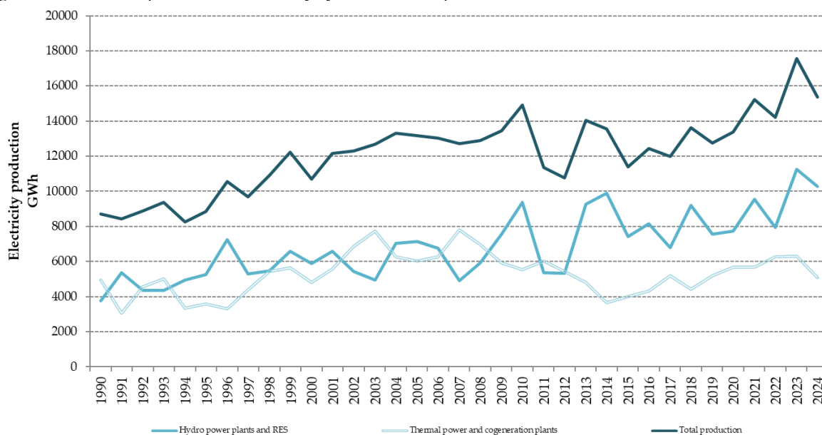
Figure 3.2-4: Domestic production of electricity by sources for the period from 1990 to 2024
