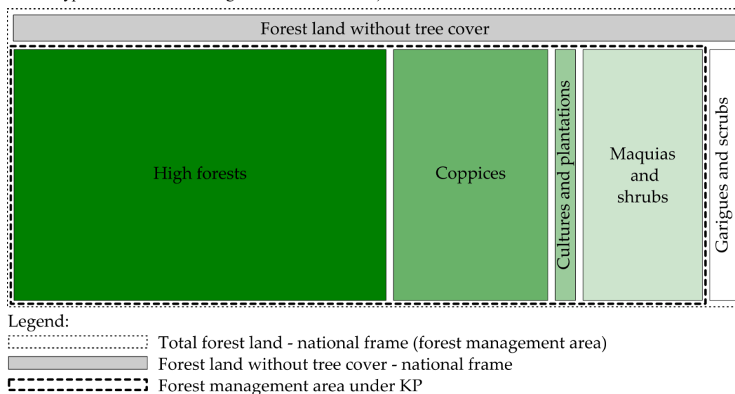
Figure 6.4-2: Forest land area under the UNFCCC and within the national framework (based on the relative share of forest types in total forest management area in Croatia)
