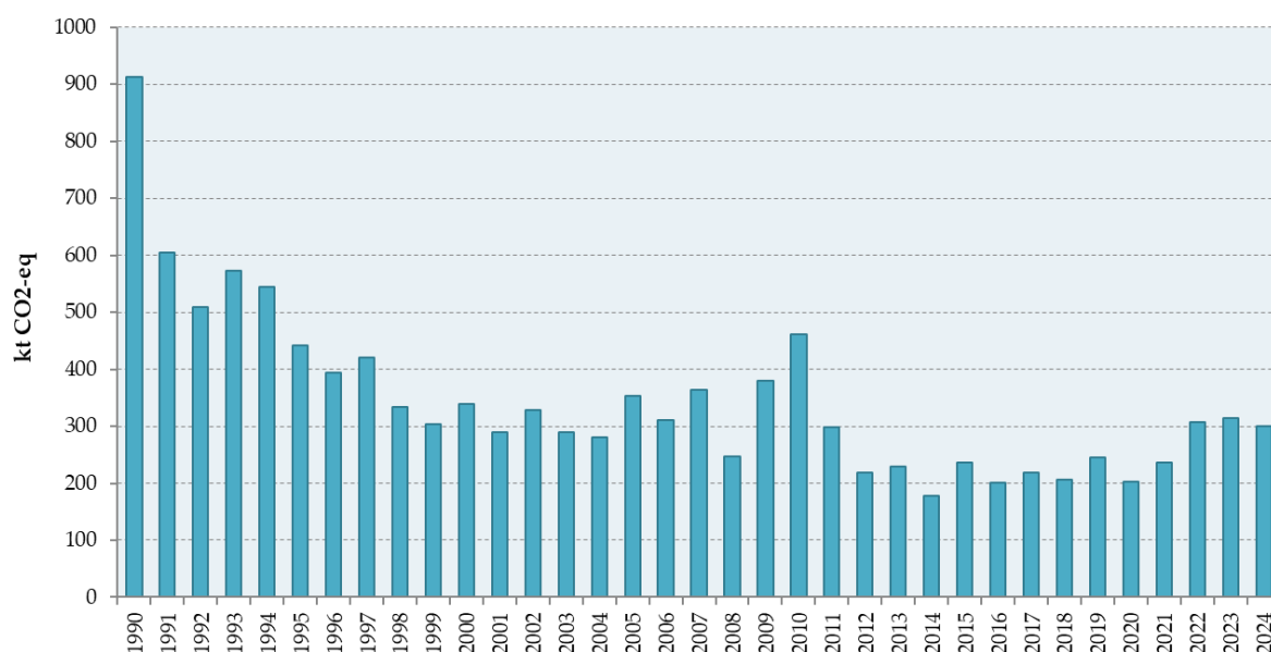
Figure 3.2-6: CO 2 -eq emissions from Manufacturing of Solid Fuels and Other Energy Industries for the period from 1990 to 2024
