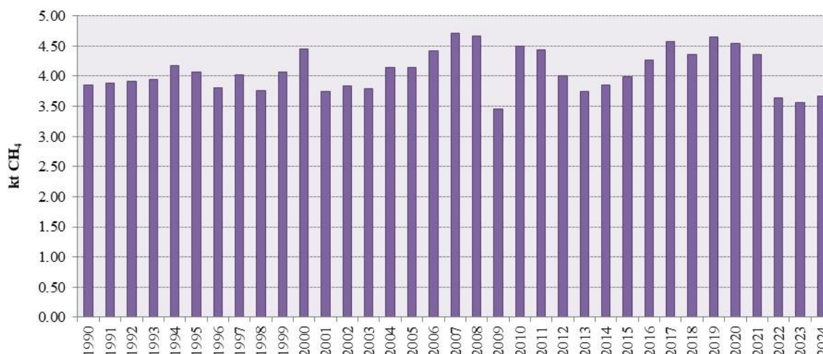
Figure 7.5-3: Emissions of CH 4 from 5.D.2 Industrial Wastewater (1990 – 2024)
