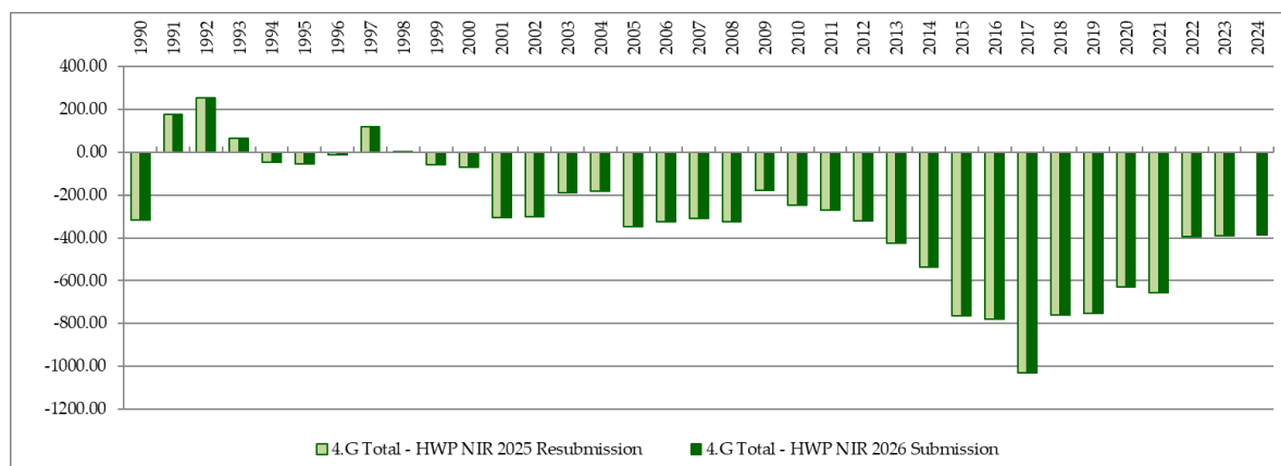
Figure 6.10-1: Current and previously reported emissions (+) and removals (-) in HWP (kt CO 2 )
