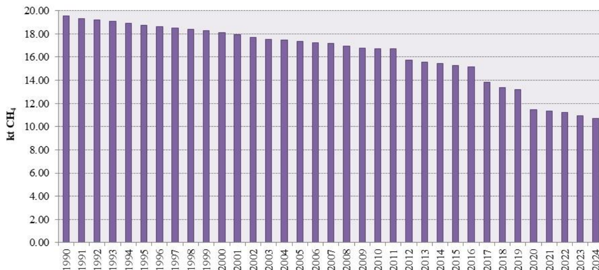
Figure 7.5-1: Emissions of CH 4 from 5.D.1 Domestic Wastewater (1990 – 2024)
