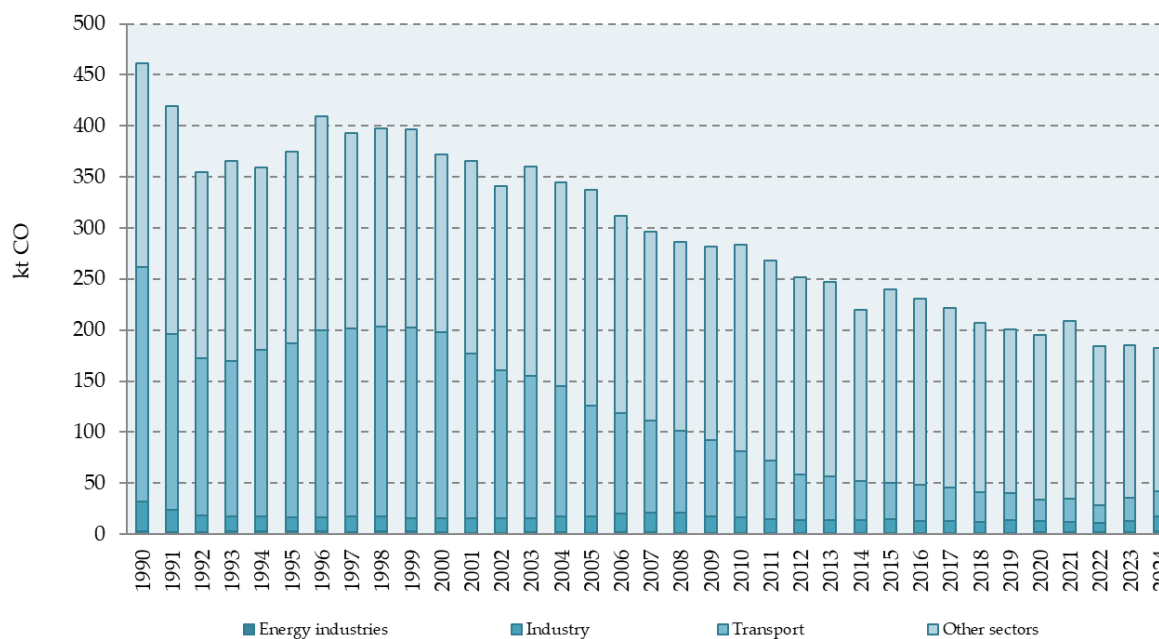
Figure 3.1-8: CO emissions from Energy sector in the period 1990-2024
