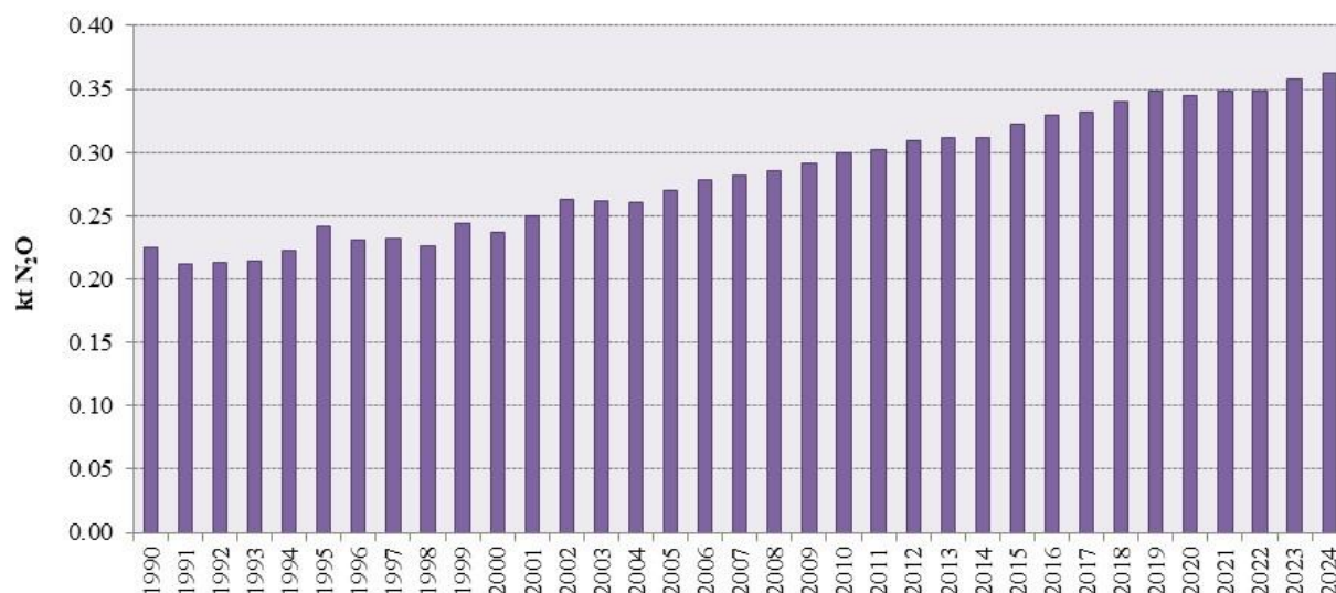
Figure 7.5-2: \text{N}_2\text{O} Emissions from Wastewater (1990 – 2024)
