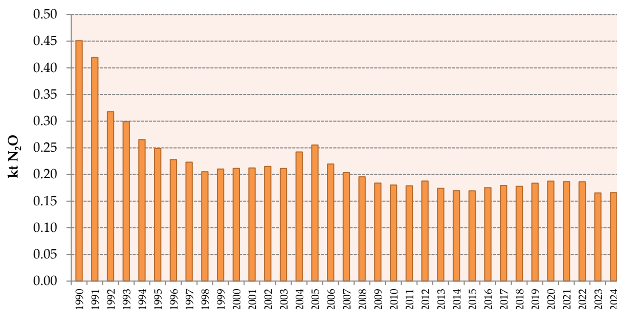
Figure 5.5-4: N_2O emissions due to urine and dung deposited by grazing animals
