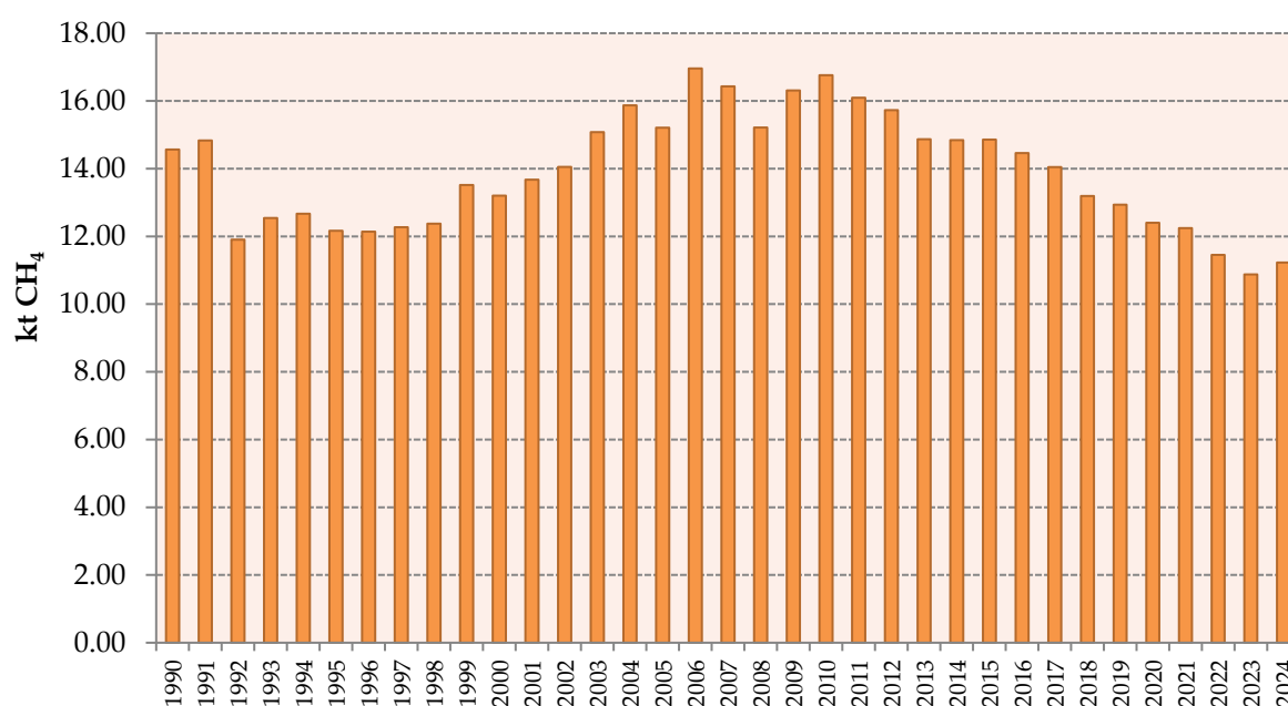
Figure 5.3-1: CH 4 emission from Manure management
