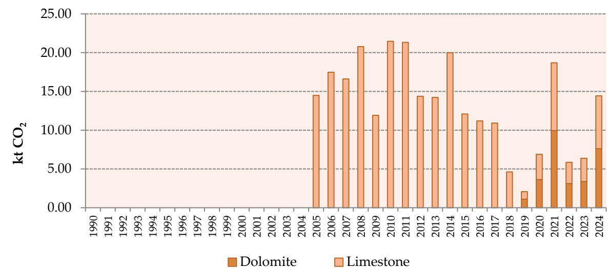
Figure 5.8-1: Direct CO 2 emissions from Liming
