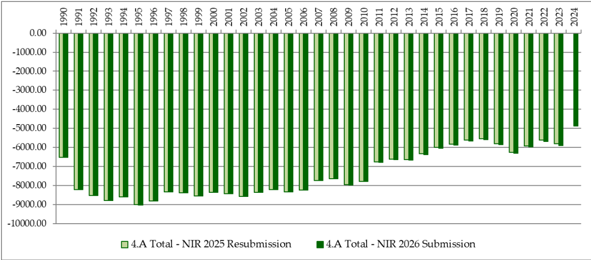
Figure 6.4-16: Current and previously reported emissions for category 4.A (kt CO 2 -eq)
