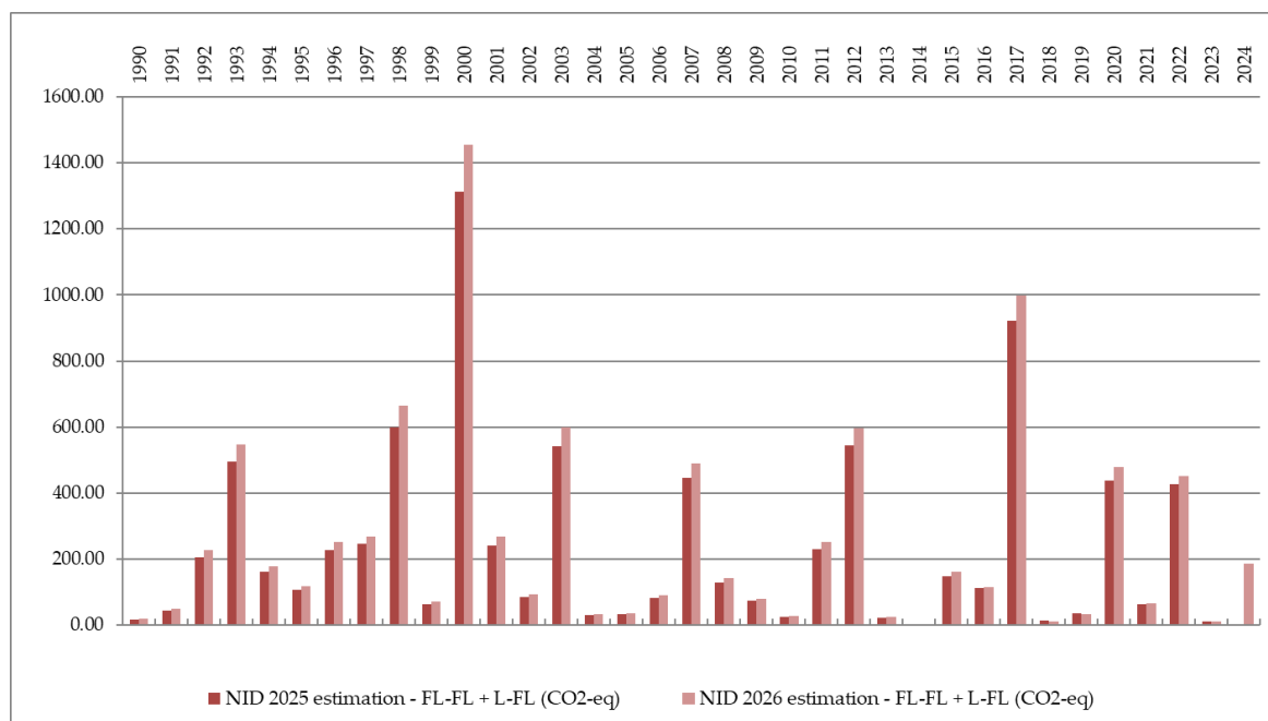
Figure 6.15-5: Recalculations of emissions (CO 2 -eq) due to forest fires per year
