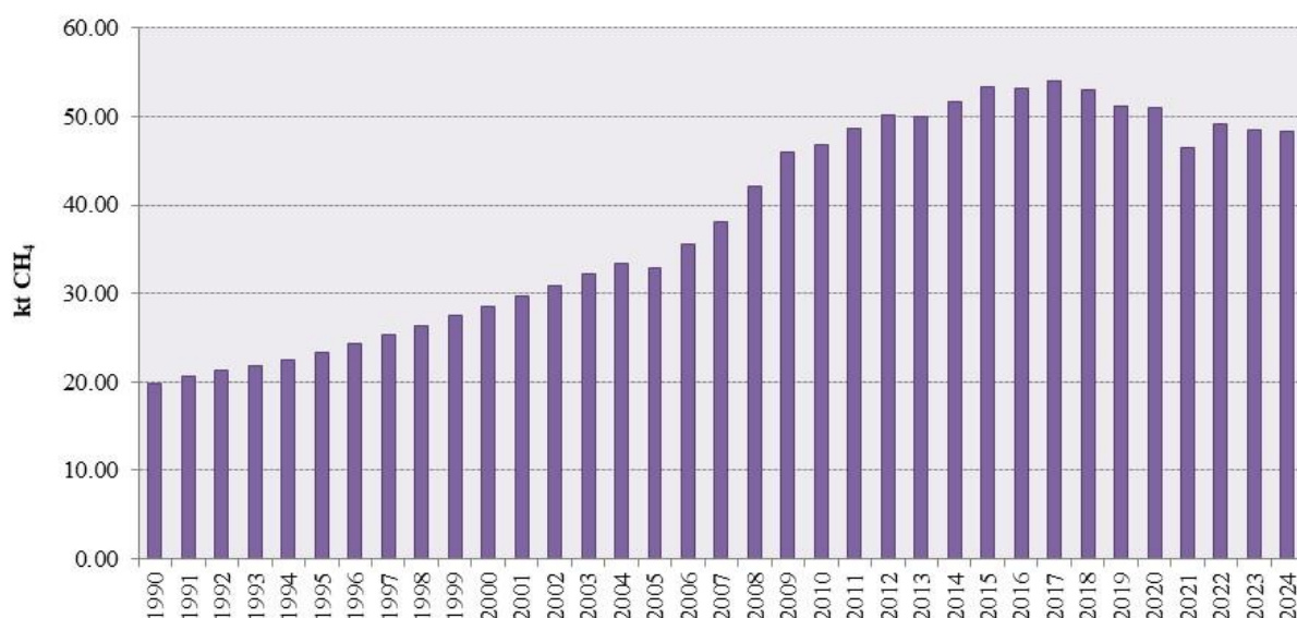
Figure 7.2-1: Emissions of CH 4 from 5.A Solid waste disposal (1990 - 2024)
